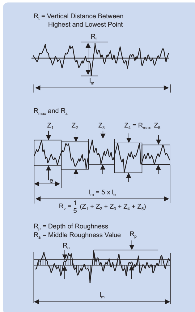
Figure 5-4: Roughness Terminology
