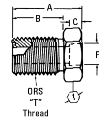
Part No. FF1922T(Size)* (Ref. SAE 520604)
