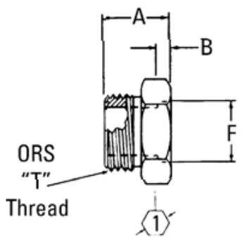
Part No. FF1851T(Size)* (Ref. SAE 520104)
